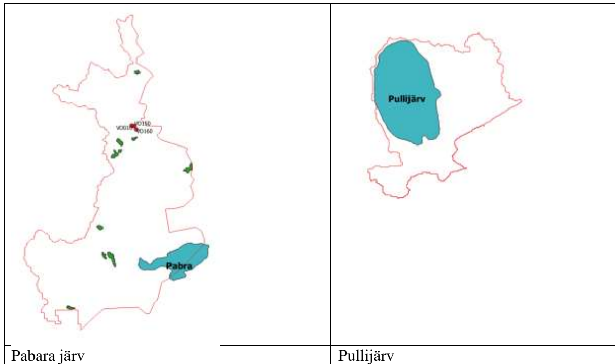
Figure 1.1 Locations of clear-cuts during 2013-2016 inside the catchment area of lakes Murati järv, Hinojärv, Kirikumäe järv, Köstrejärv, Aherujärv, Ähijärv, Pabra järv and Pullijärv. Red dots are locations of waste-water outlets in catchment area of Lake Pabra and Köstrejärv.
